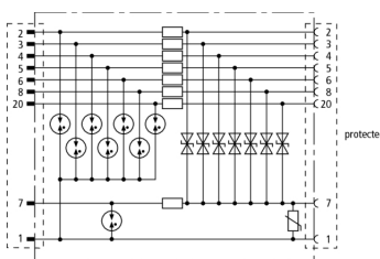
Basic circuit diagram USD 25 V24 HS S B
