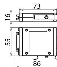
Dimension drawing USD 25 V24 HS S B
